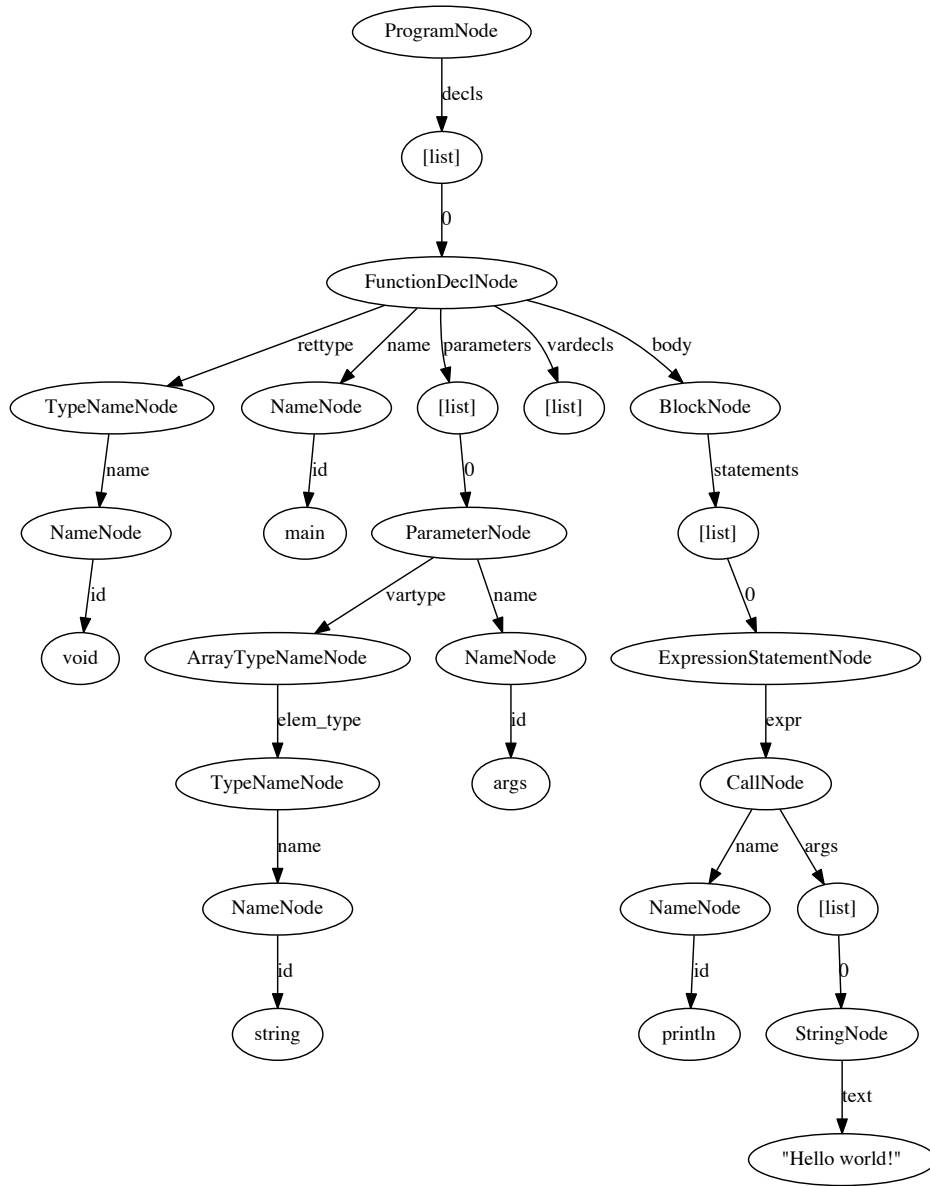
Figure 1: AST for a small uC program.
